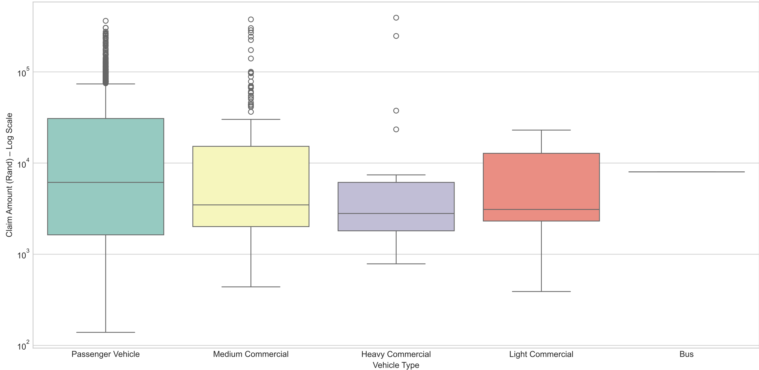
Claim Amount Distribution by Vehicle Type
