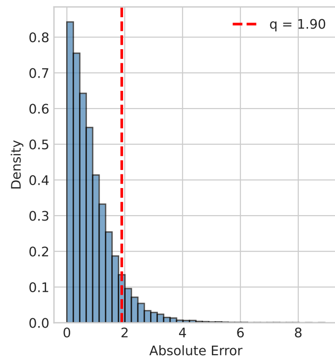
E. Error Distribution
