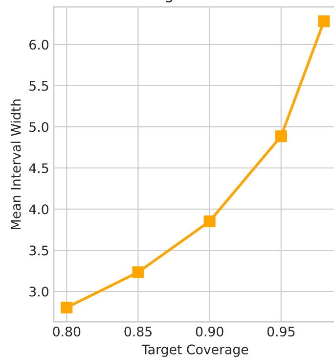
C. Coverage-Width Tradeoff
