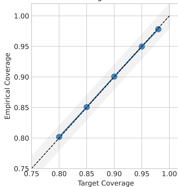
B. Coverage Calibration
