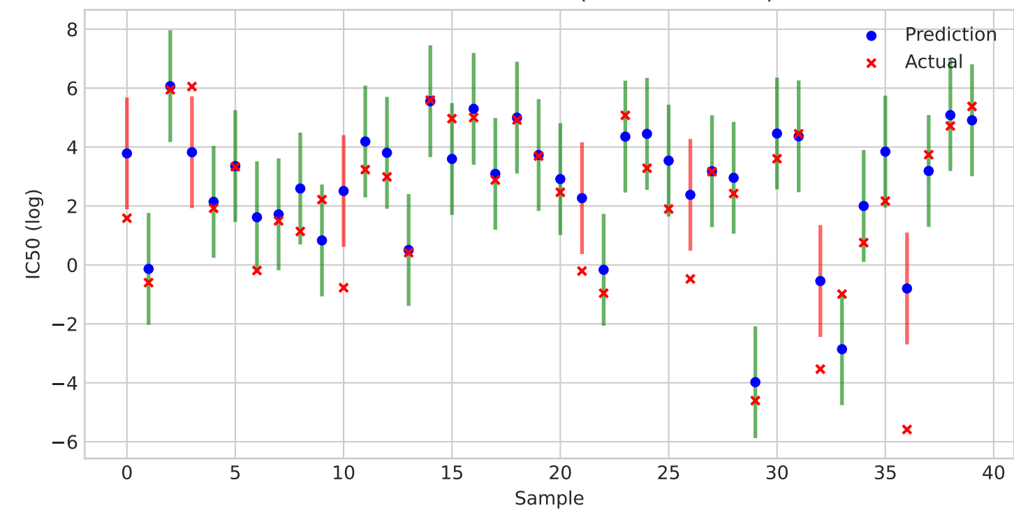
D. Prediction Intervals (90% confidence)
