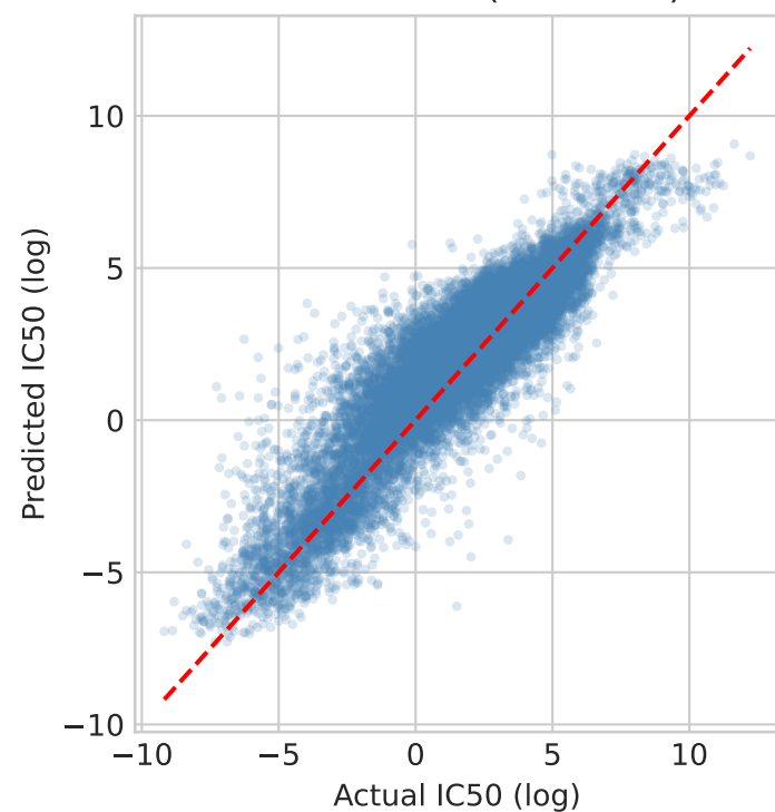
A. Predictions ( r = 0.909 )
