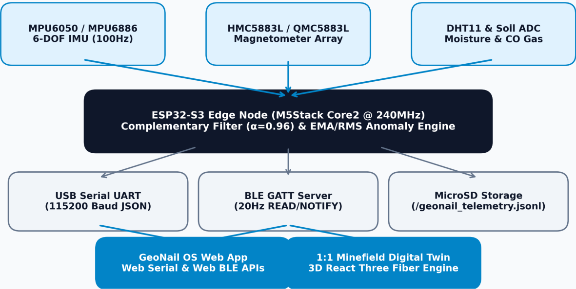
FIGURE 1: END-TO-END GEONAIL DATA PIPELINE & SUBSYSTEM ARCHITECTURE
