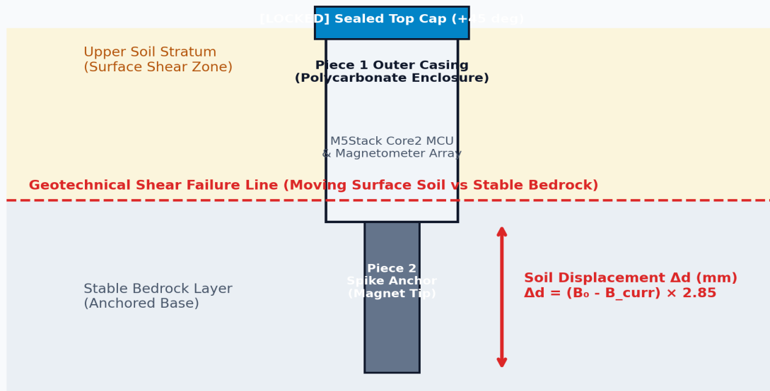
FIGURE 3: GEONAIL SUBTERRANEAN KINEMATIC & ANCHOR DISPLACEMENT MECHANISM
