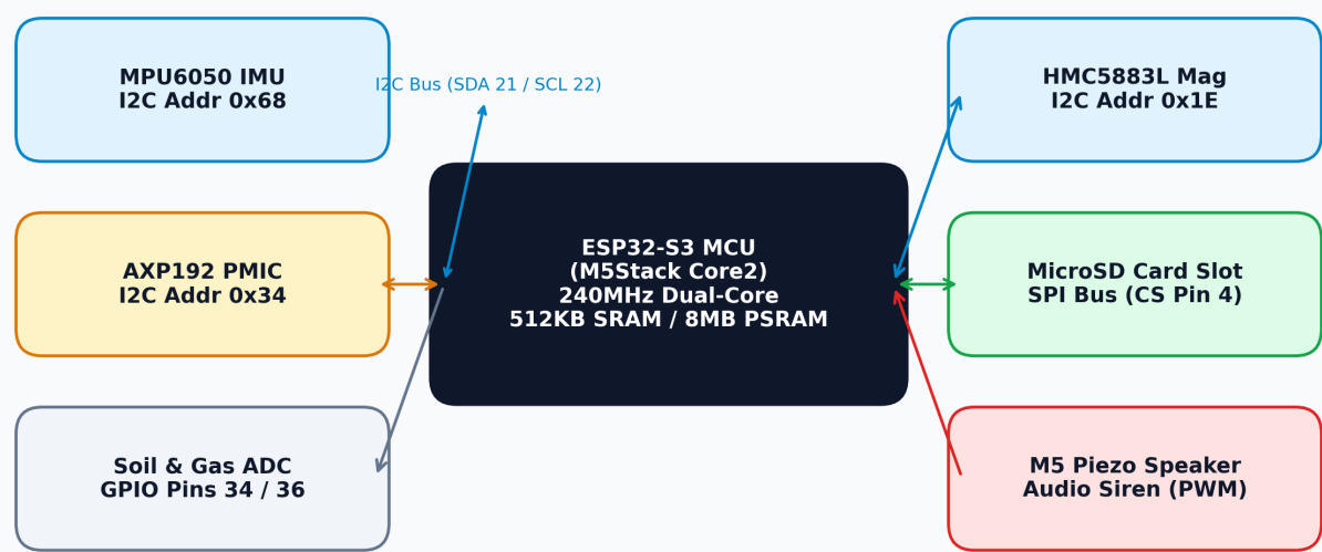
FIGURE 2: ESP32-S3 HARDWARE INTERFACE & BUS ARCHITECTURE
