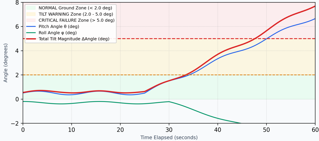
FIGURE 5: REAL-TIME SENSOR ORIENTATION & TILT ANGLE HISTORY (60s WINDOW)
