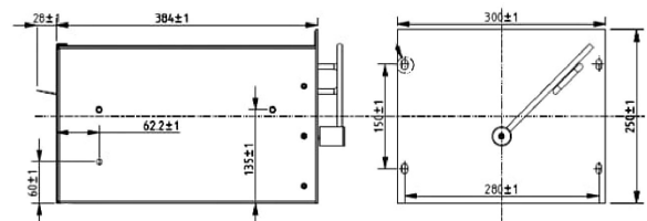
8-Pole, 63 A, 750V
