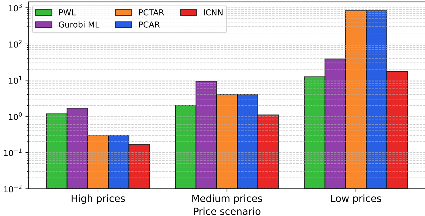
Mean optimality gap vs Exact NLP (%, log-scale)
