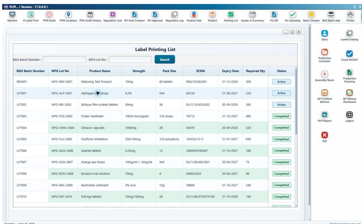
Figure 10 - Label Printing queue with common search fields and controlled batch status
