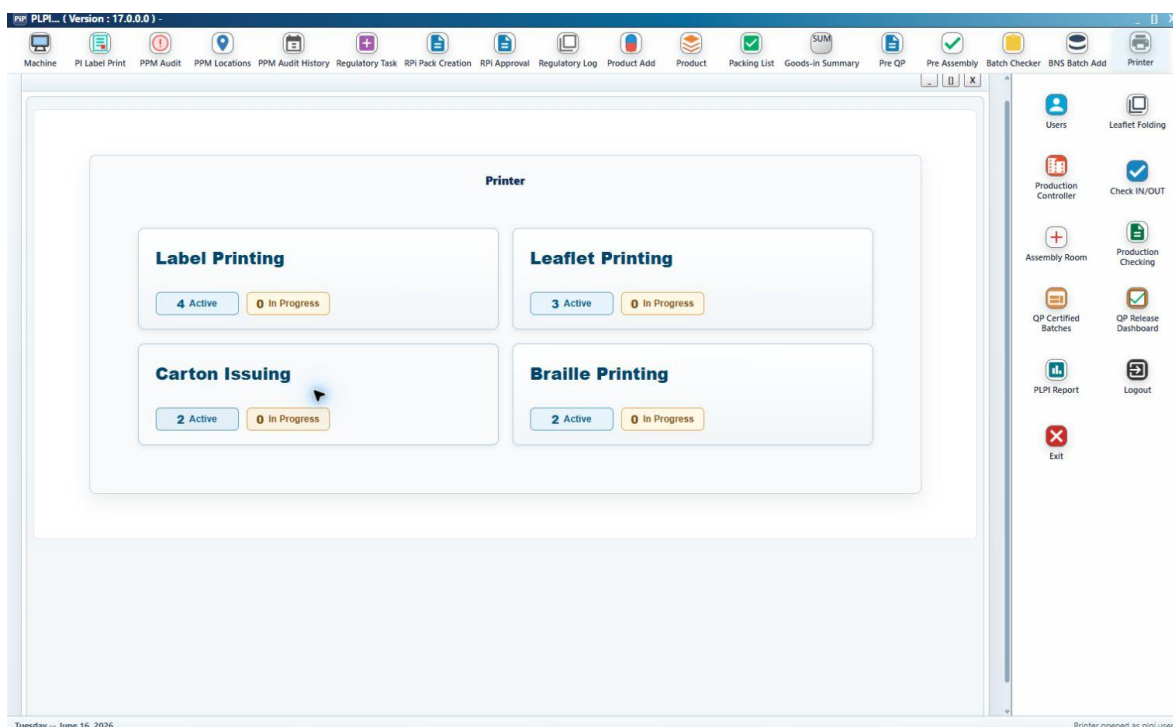
Figure 15 - Carton Issuing queue for eligible Reboxing batches
