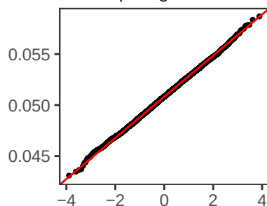
Prop MM
