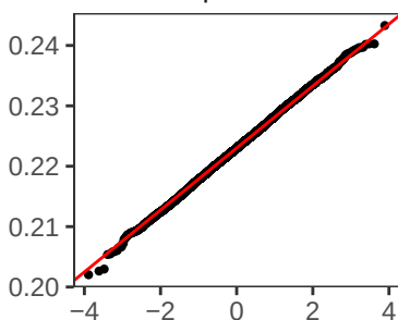
Prop School
