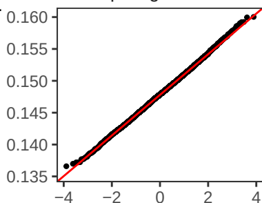
Prop School
