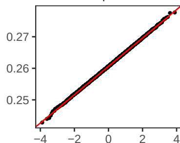
Prop MM
