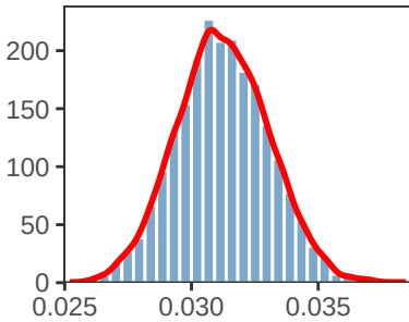
Prop Tertiary
