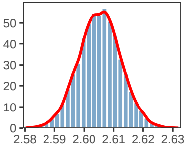
Prop Age 20-35
