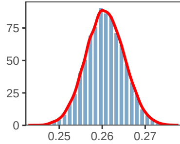
Prop Secondary
