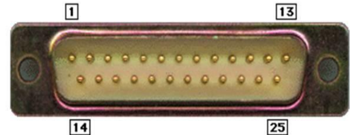
DB-25 Male (DCE side)
