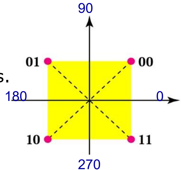
QPSK(4-PSK) 1 amplitude 4 phases
