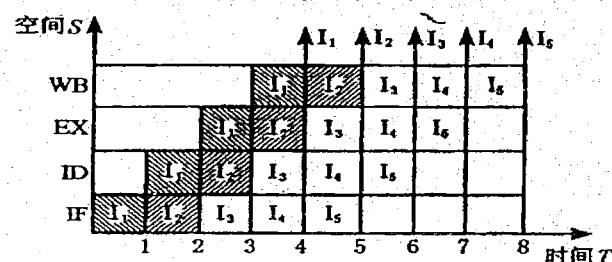
(c)流水 CPU 时空图
