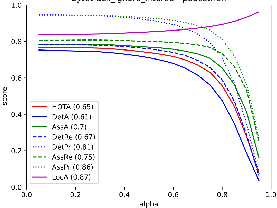
bytetrack_ignore_filtered - pedestrian
