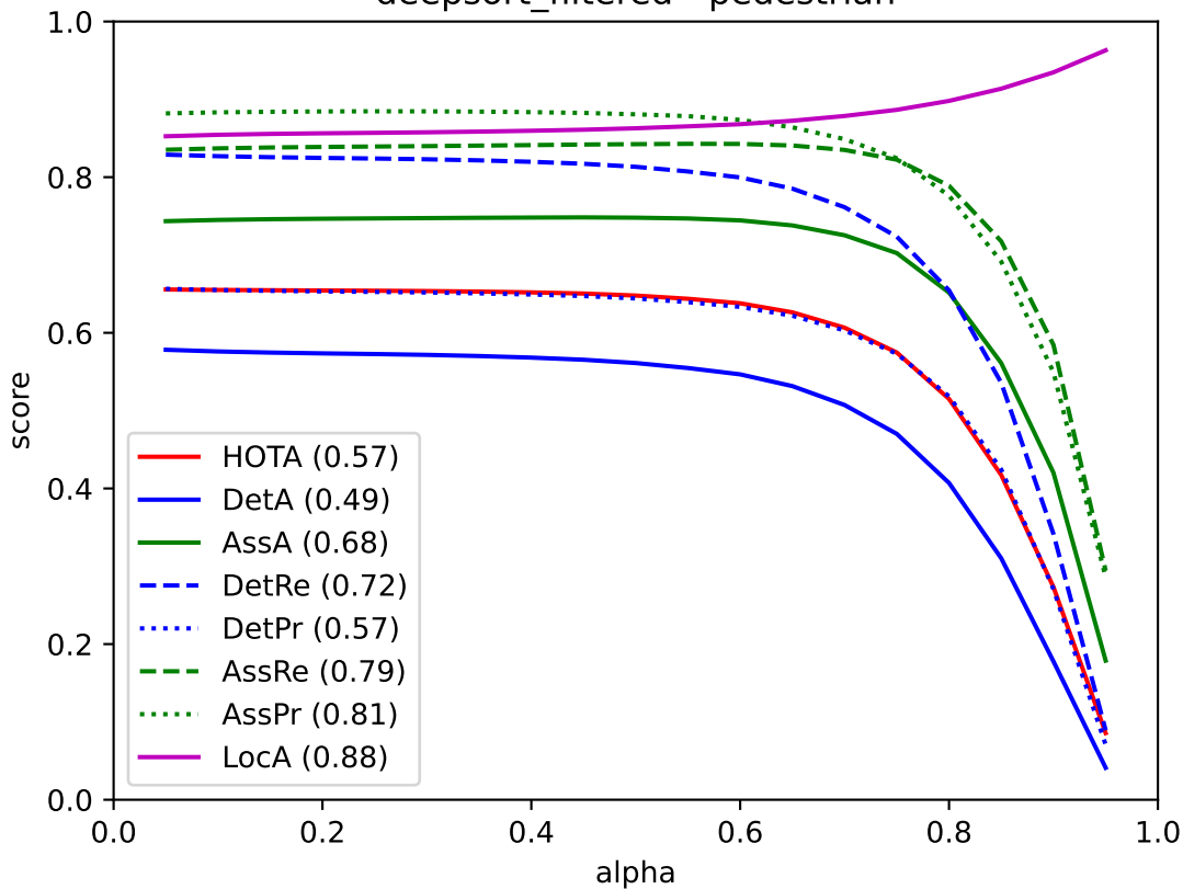
deepsort_filtered - pedestrian
