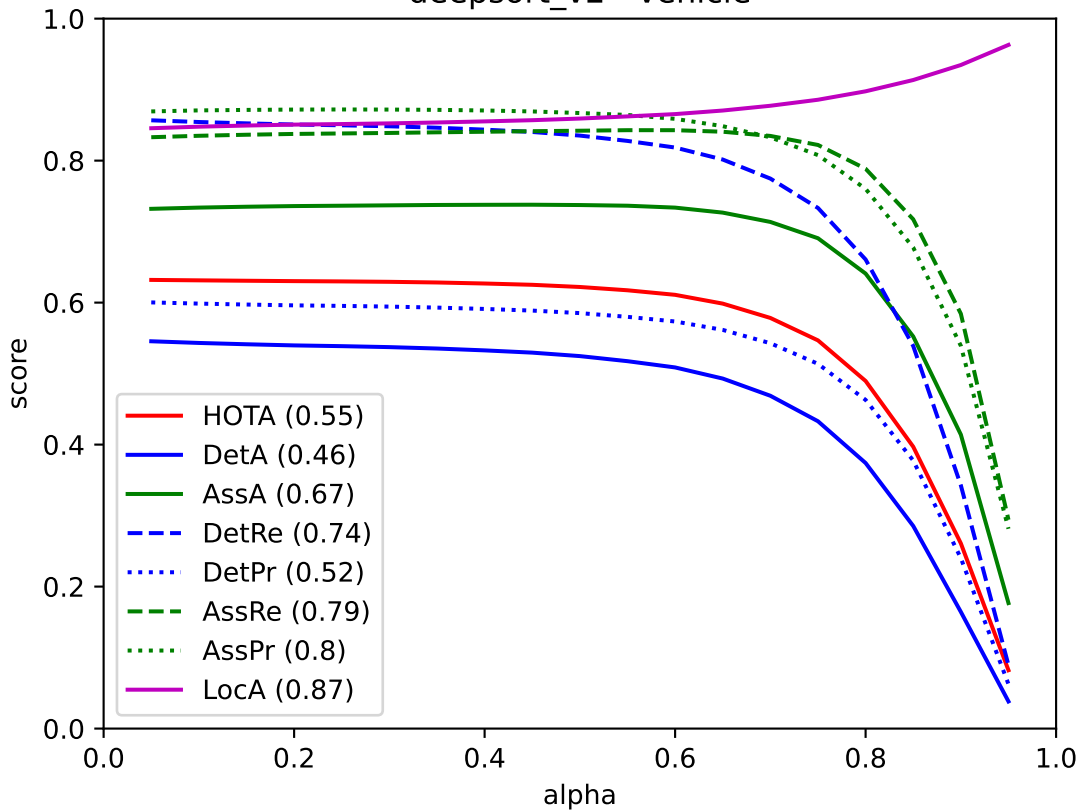
deepsort_v2 - vehicle
