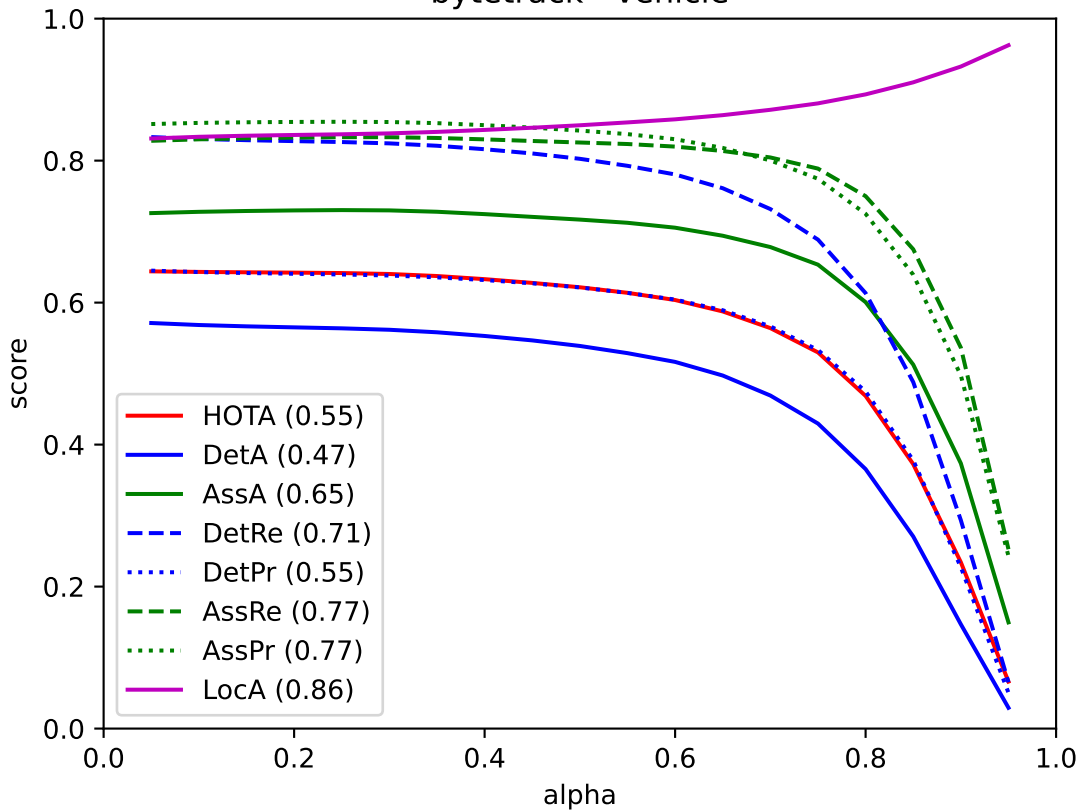
bytetrack - vehicle
