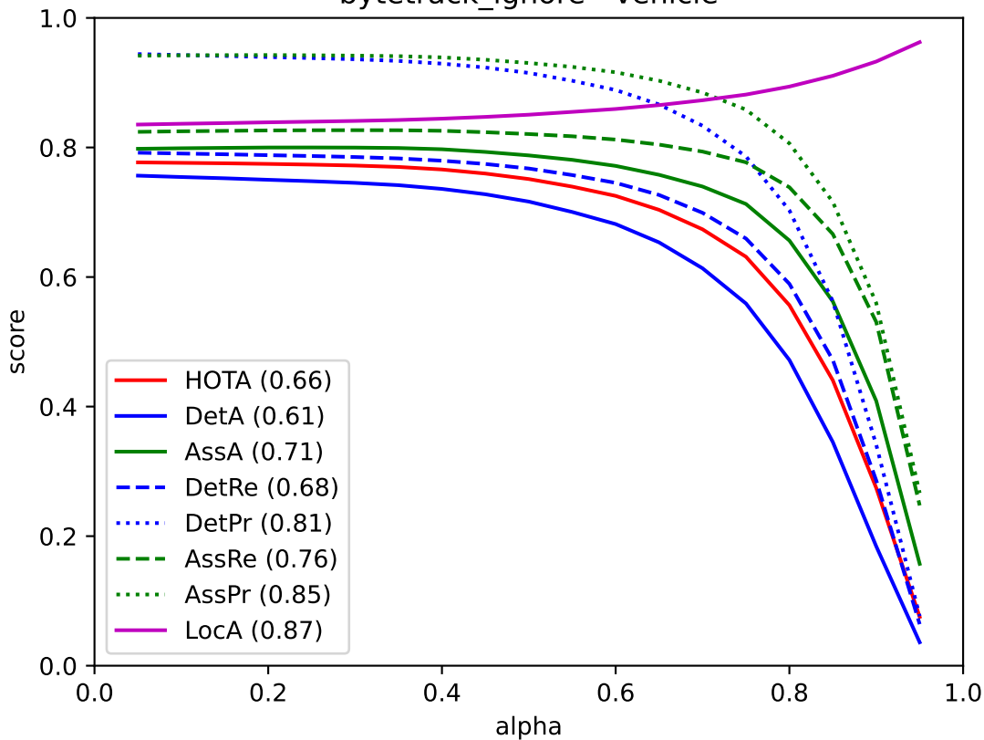
bytetrack_ignore - vehicle
