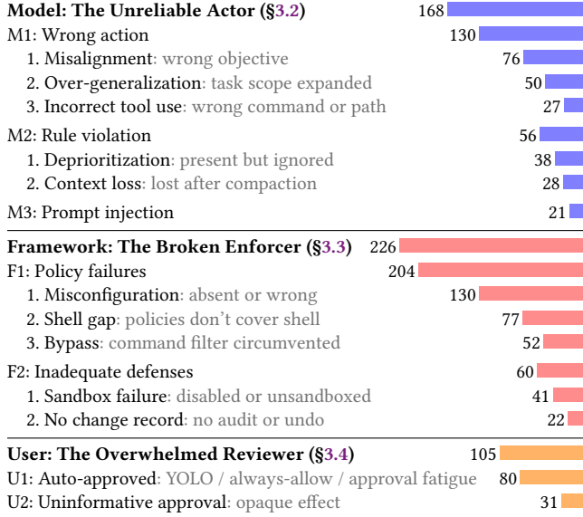
Figure 4. Taxonomy of causes. Counts can overlap.
