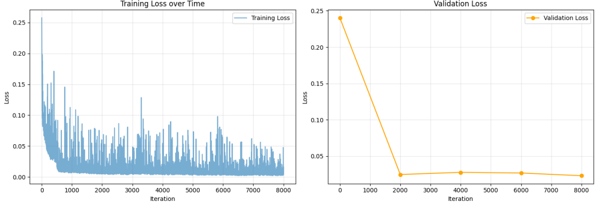
Figure 8.2: FFKSM training convergence: (left) training MSE loss trajectory over 150 epochs; (right) validation loss confirming stable generalization without overfitting.
