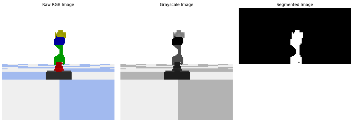
Figure 3.3: Data preprocessing pipeline: RGB image acquisition, grayscale conversion, and binary segmentation to produce silhouette masks.
