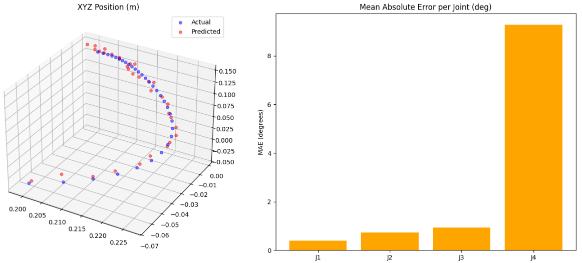
Figure 8.1: Multi-view NeuroKin-3D diagnostics: (left) 3D cloud of predicted vs. ground-truth end-effector positions; (right) per-joint mean absolute error for all four joints.
