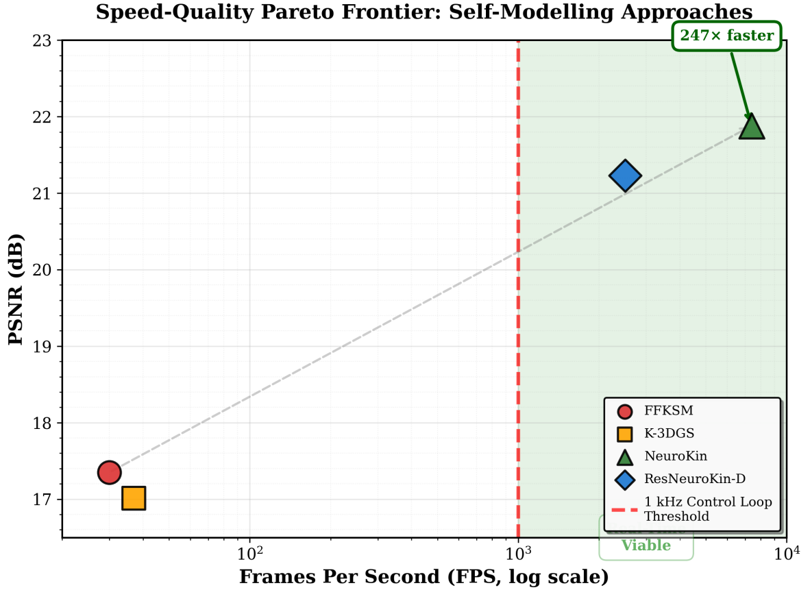
Figure 7.1: Pareto frontier of self-modeling architectures: inference speed vs. reconstruction quality (PSNR), highlighting control-oriented trade-offs of direct decoding vs. volumetric rendering.
