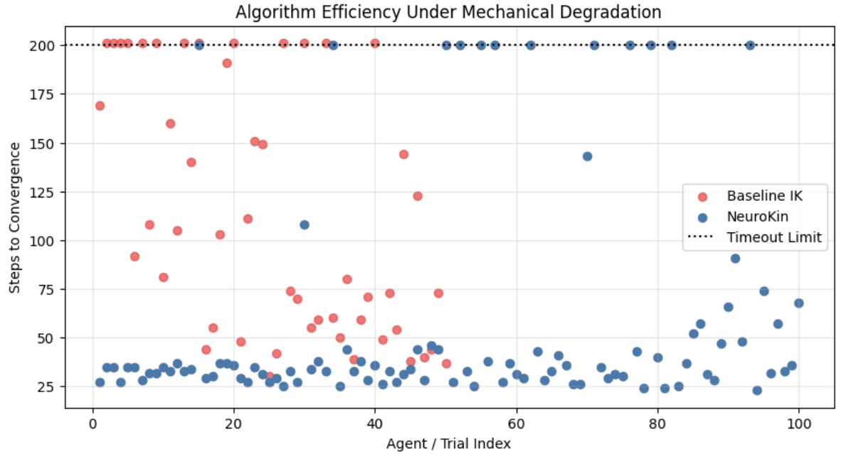
Figure 6.3: A comparative scatter plot charting the number of control steps taken across 100 individual trials, contrasting Baseline method performance against the Neurokin method.
