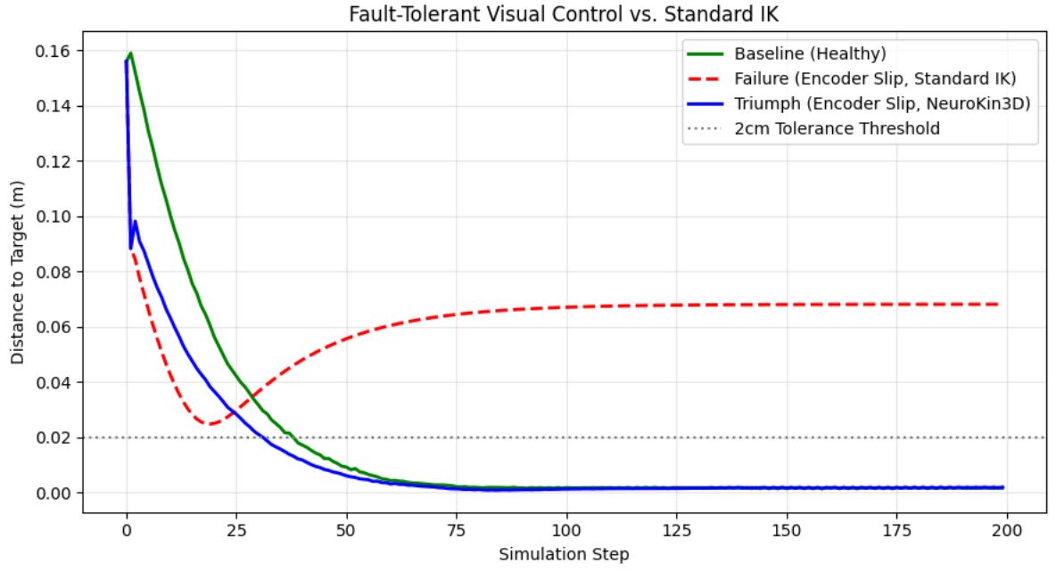
Figure 5.5: Dynamic error recovery following actuator fault injection. The blind baseline controller diverges catastrophically, while NeuroKin’s visual estimates enable rapid re-convergence to the target.
