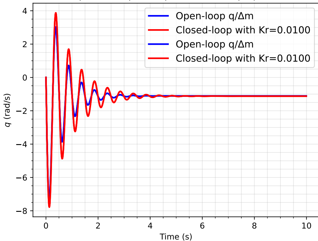
Comparison: Open-loop vs Closed-loop ( \xi = 0.65 )
