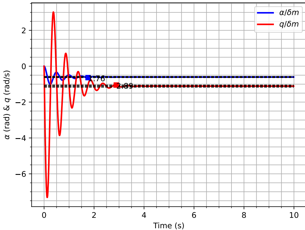
Step response \alpha/\delta m et q/\delta m
