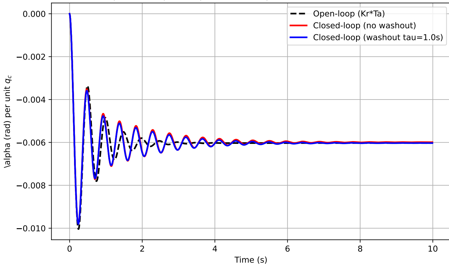
Comparison: Open-loop / Closed-loop without filter / with washout
