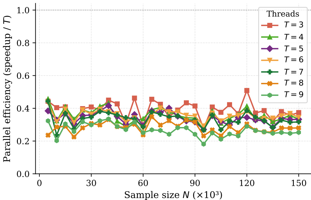
Newton's method
