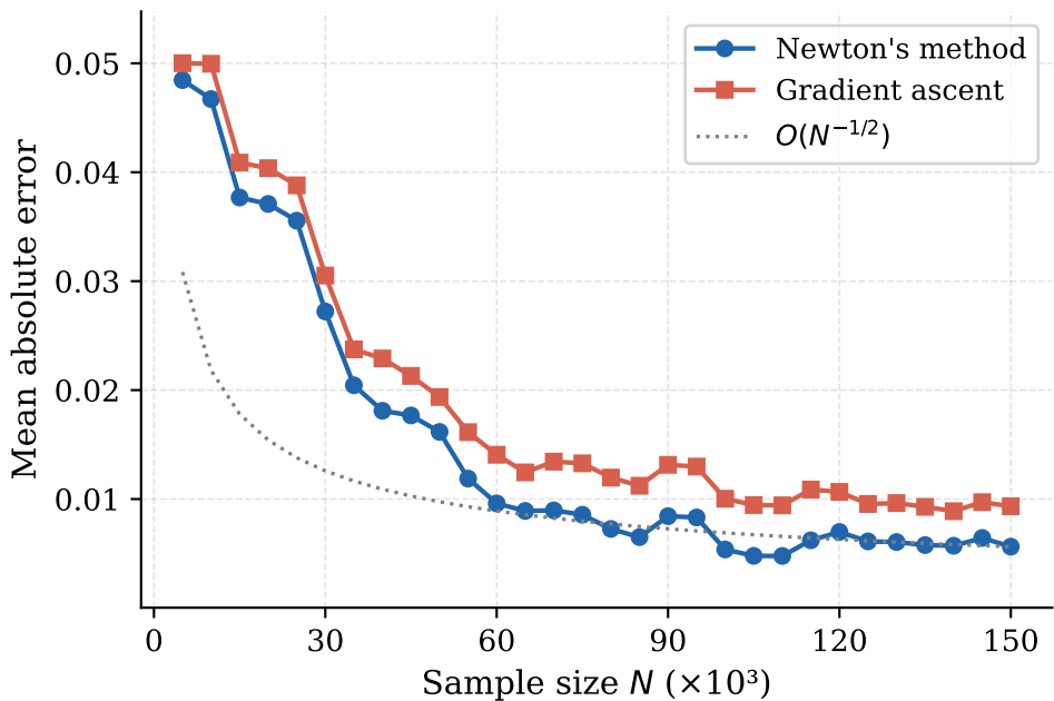
MAE vs. N — parallel — p = 5 , d = 2 , T = 8
