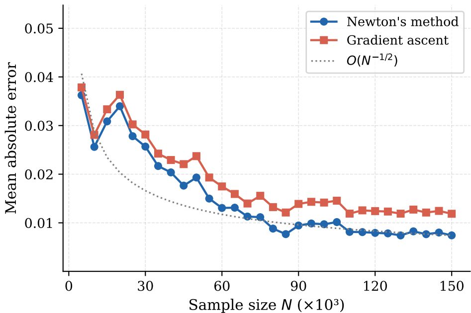
MAE vs. N — sequential — p = 5 , d = 2
