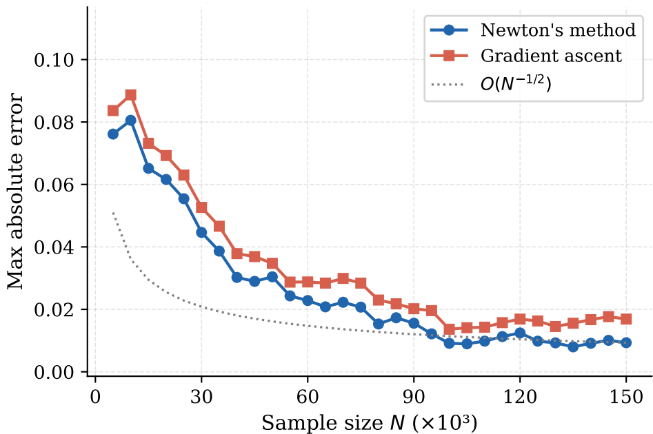
Max AE vs. N — parallel — p = 5, d = 2, T = 8
