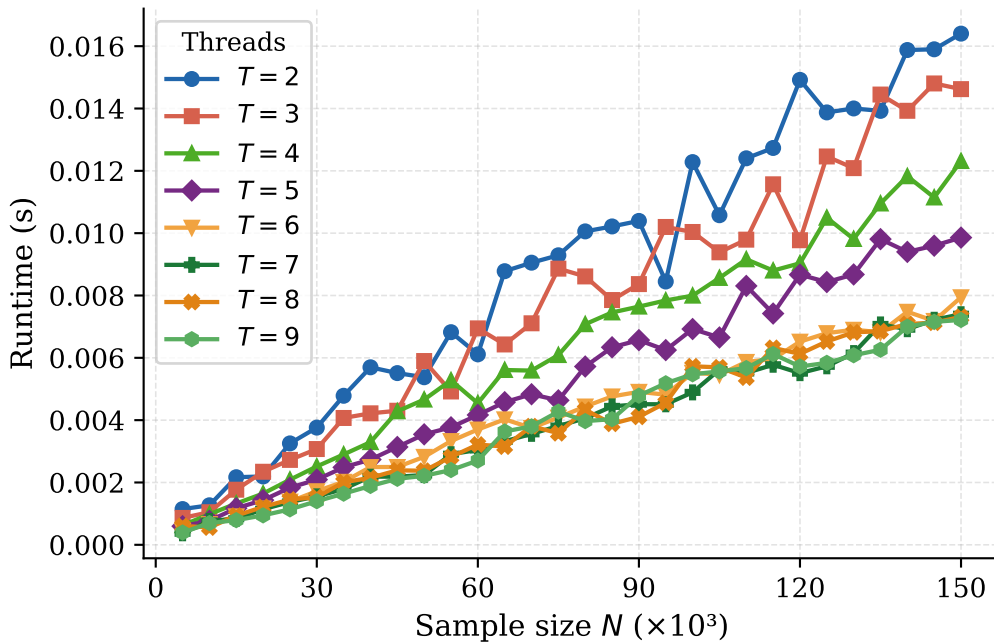
Newton's method
