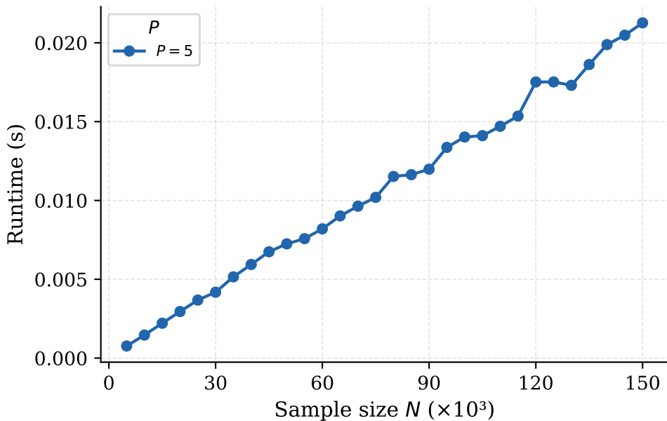
Newton's method
