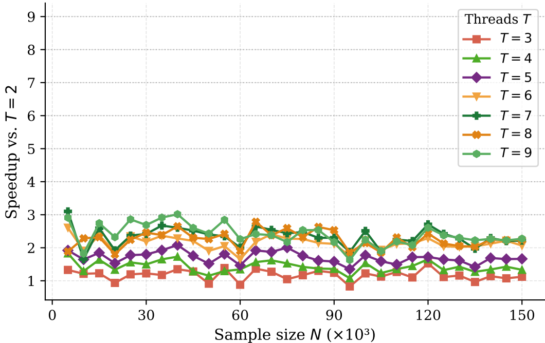
Parallel speedup — Newton's method
