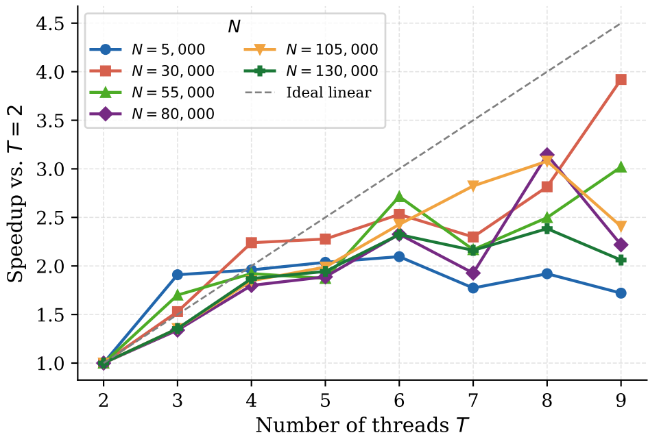
Speedup vs. thread count — Gradient ascent
