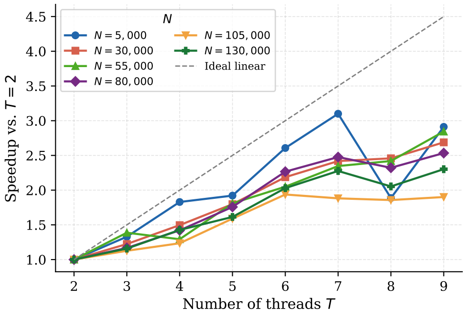
Speedup vs. thread count — Newton's method
