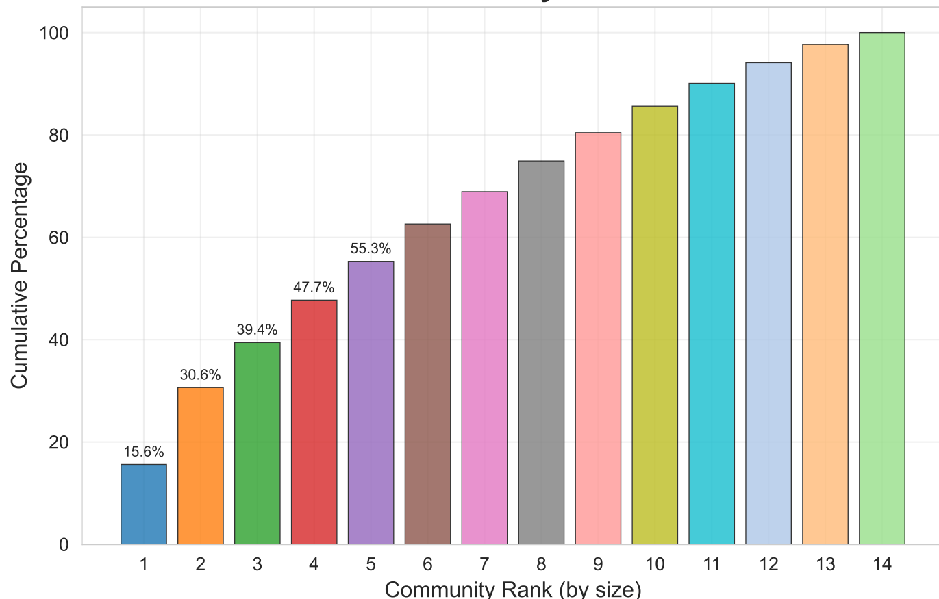
Cumulative Community Size Distribution
