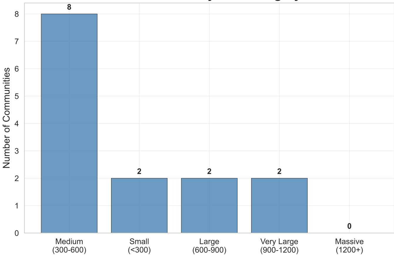
Communities by Size Category
