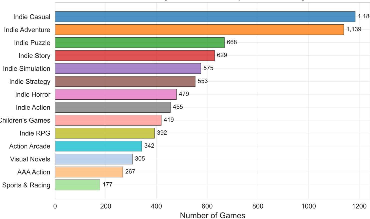
Community Sizes - Games per Community
