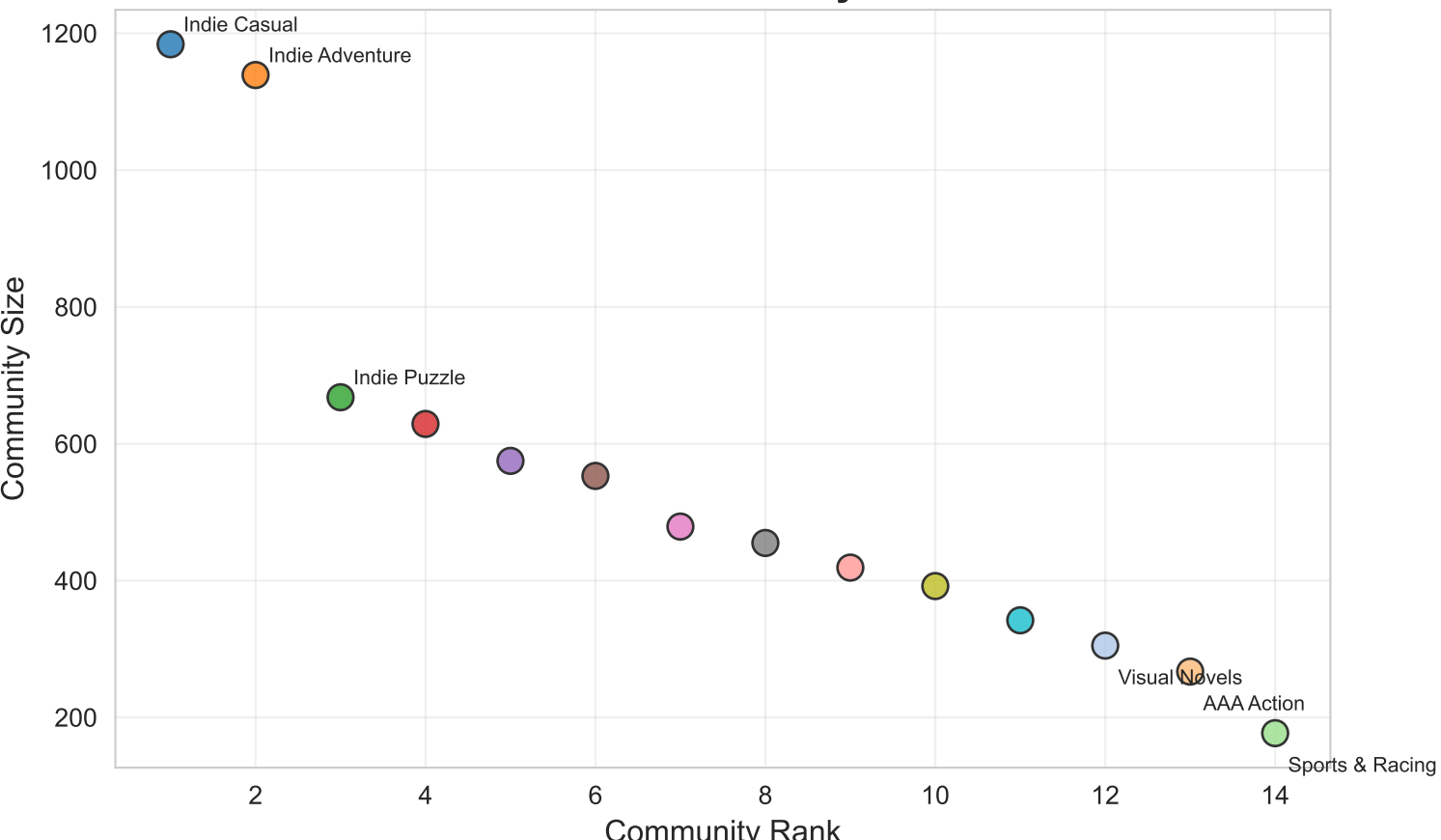
Size Distribution by Rank
