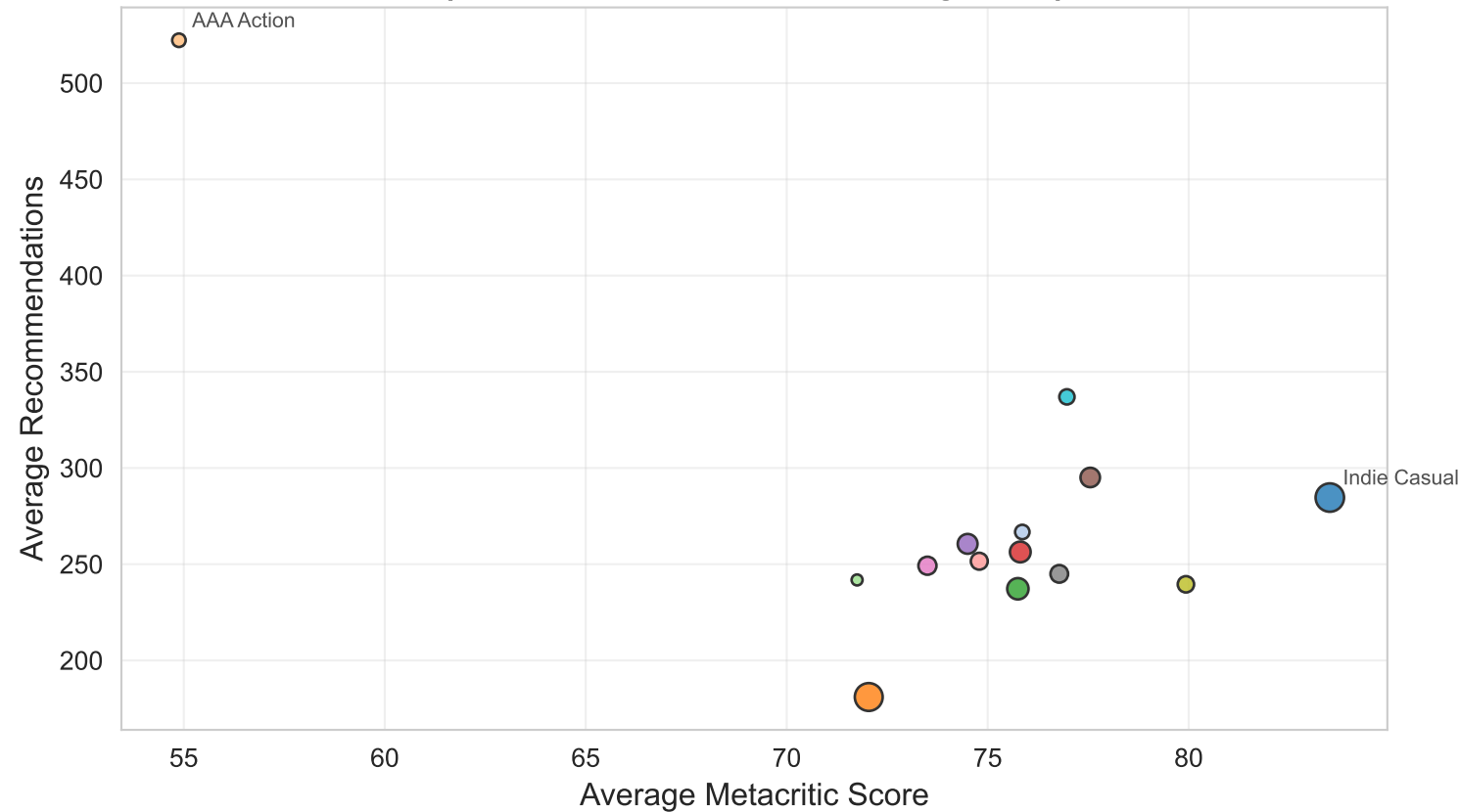
Quality vs Popularity (Bubble size = Community size)
