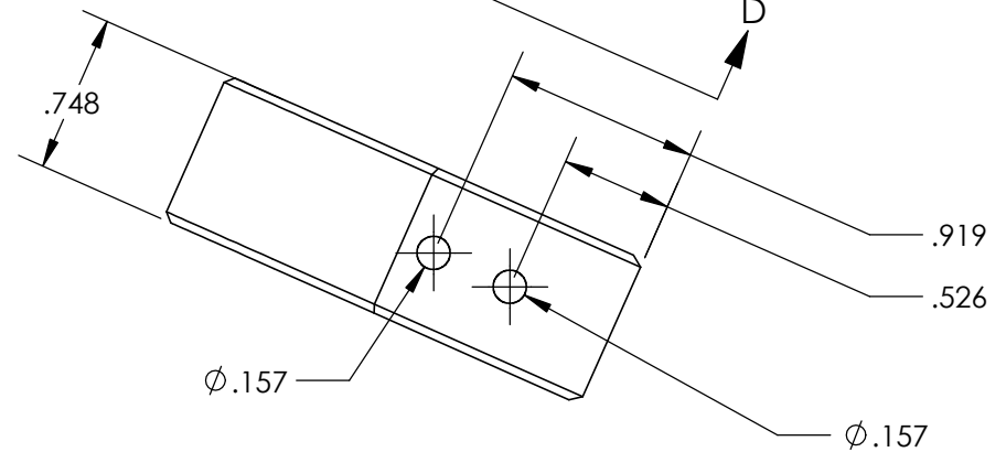
VIEW D-D
