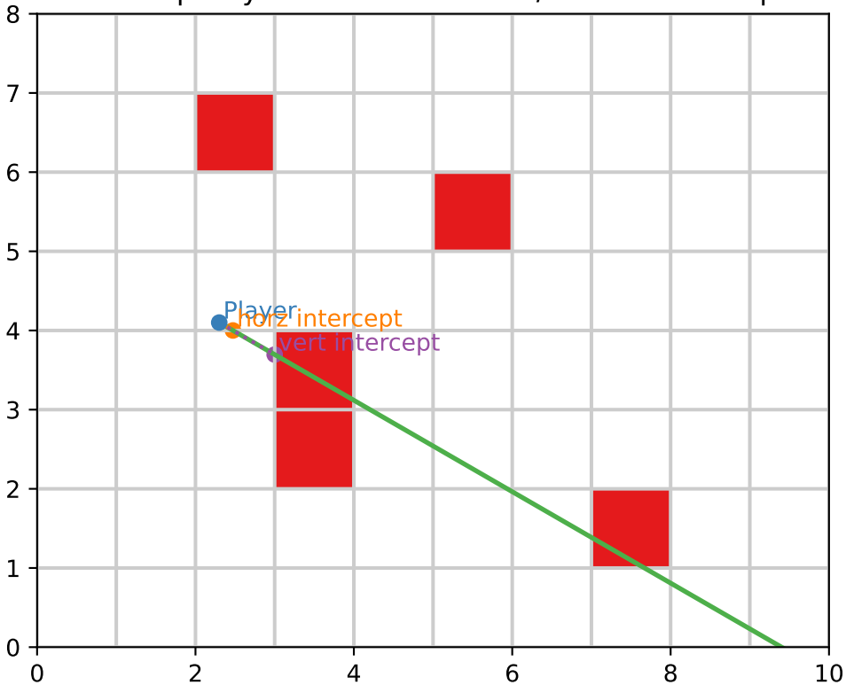
Grid map: ray and first horizontal/vertical intercepts
