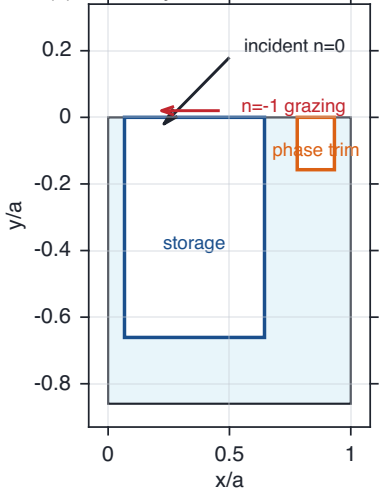
(a) two-cavity radiation-control unit cell
