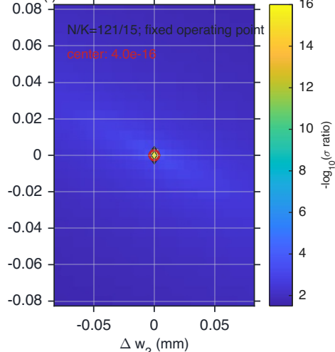
(f) fixed-root fabrication tolerance
