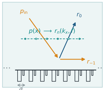
a Bloch-wave scattering
