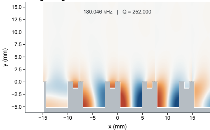
a High-Q eigenmode
