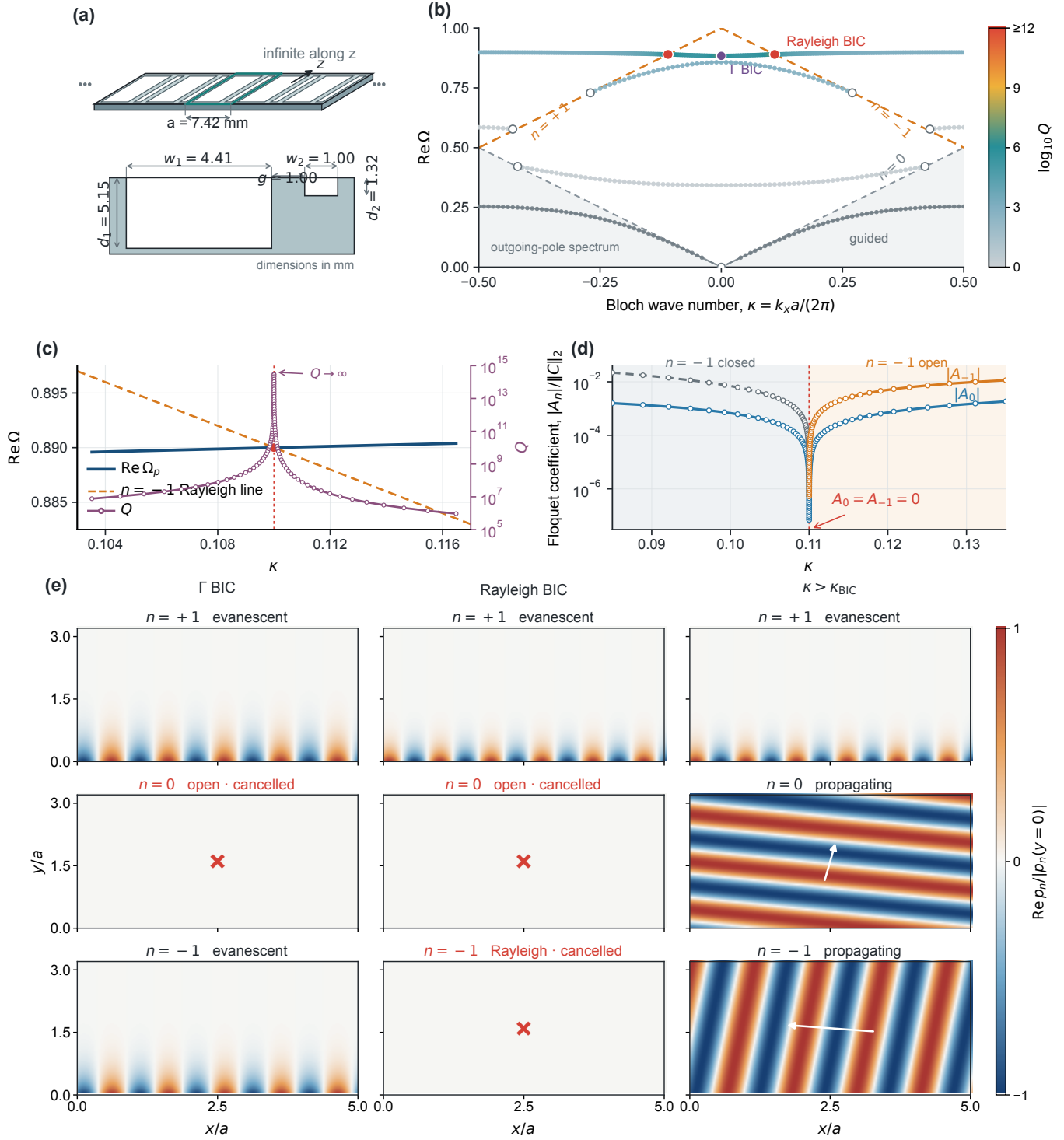
FIG. 2. Rayleigh BIC in an underwater acoustic metagrating. (a) Periodic two-groove surface and unit-cell dimensions. (b) Outgoing-pole spectrum; color gives \log_{10} Q , with vivid colors denoting high Q . Background poles are joined only over locally continuous, channel-consistent segments; open circles mark terminations at square-root cuts. The purple point is a symmetry-protected \Gamma BIC, whereas the red points mark the reciprocal Rayleigh-BIC pair. (c) Local branch: \text{Re}\Omega_p reaches the n = -1 Rayleigh line as Q diverges. (d) Homogeneous Floquet pressure amplitudes: A_0 and A_{-1} vanish together. (e) Order-resolved exterior eigenfields at the \Gamma BIC, the Rayleigh BIC, and beyond the opening.
