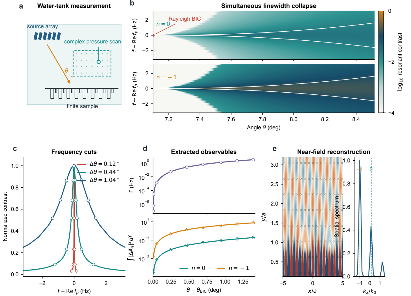
FIG. 4. Observable scattering signatures. (a) Water-tank complex-field mapping. (b) Simultaneous collapse of the background-subtracted n = 0 and n = -1 scattering linewidths; white curves denote the pole half-linewidth. (c) Physical-frequency cuts of the normalized specular resonant contrast. (d) Extracted pole linewidth and integrated spectral weights of the two propagating orders. (e) Reference-subtracted complex-field sampling and Floquet reconstruction at a nearby driven state; an exact BIC cannot be excited by the external plane wave. Open symbols and the sampled field are theory subsamples reserved for future measured data.
