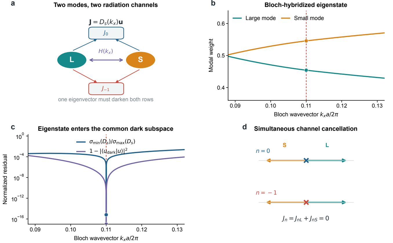
FIG. 3. Common-dark-state origin of the Rayleigh BIC. (a) Two hybrid cavity coordinates radiate into the n = 0 and n = -1 rows. (b) Bloch evolution of the large- and small-cavity modal weights. (c) Simultaneous collapse of the radiation-matrix singular-value ratio and the eigenstate-dark-state misalignment. (d) At the BIC, the two groove contributions cancel as complex phasors in both radiation rows. The strict pressure zeros are obtained from the full eigenproblem in Fig. 2.
