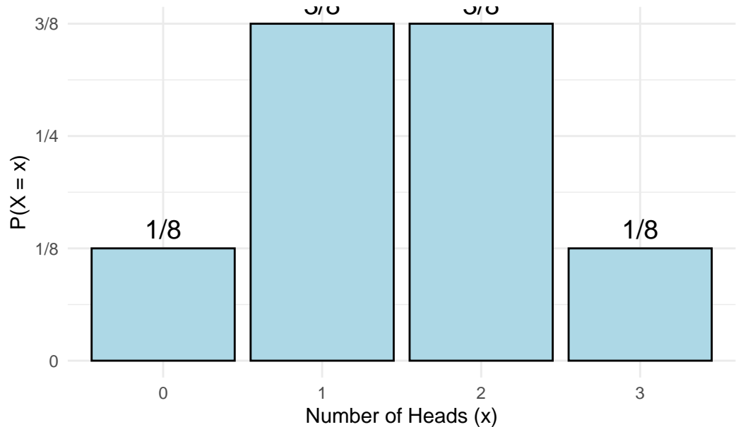
PMF of Number of Heads in 3 Tosses
