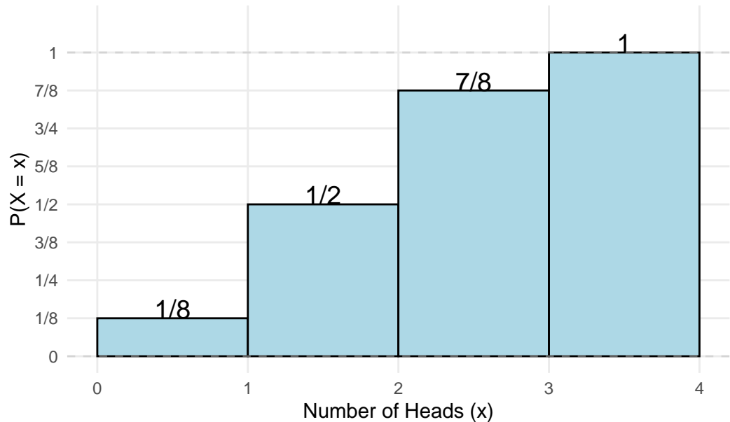
CDF of Number of Heads in 3 Tosses
