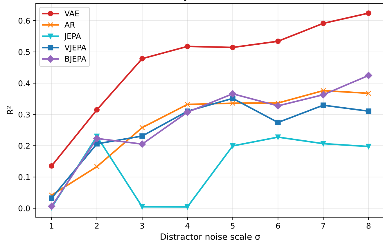
Noise Recovery (Test) [MLP backbone]
