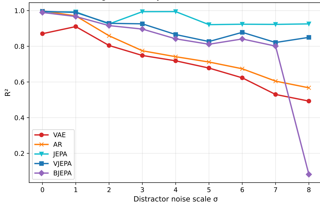
Signal Recovery (Test) [MLP backbone]
