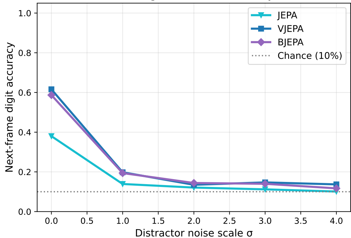
Test Digit Prediction Accuracy
