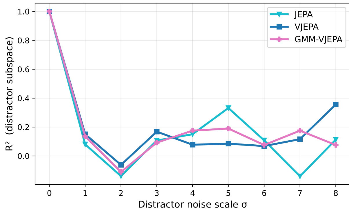
Noise Recovery (Test Set) Lower is better
