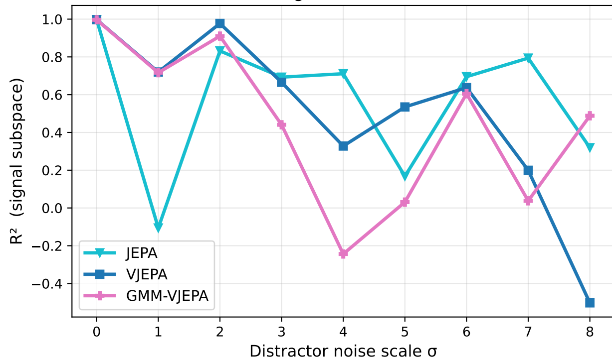
Signal Recovery (Test Set) Higher is better
