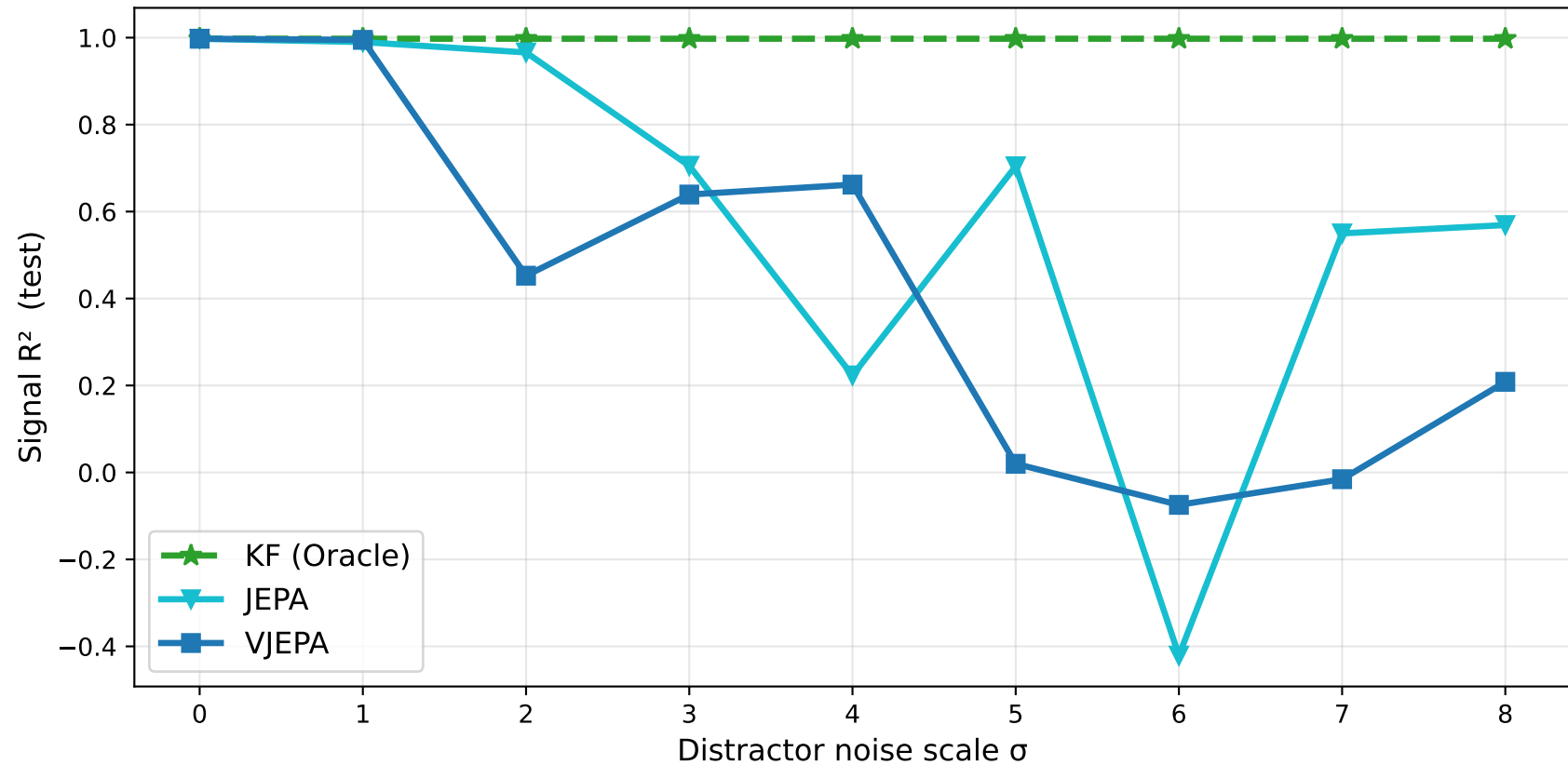
Experiment 5: Oracle Kalman Filter vs. JEPA / VJEPA Signal subspace R^2 (test set; KF = theoretical upper bound)
