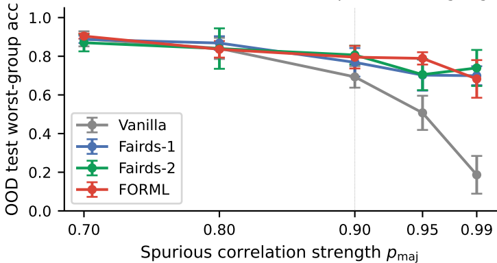
Phase transition: Fairds-2 robust as spurious strength grows
