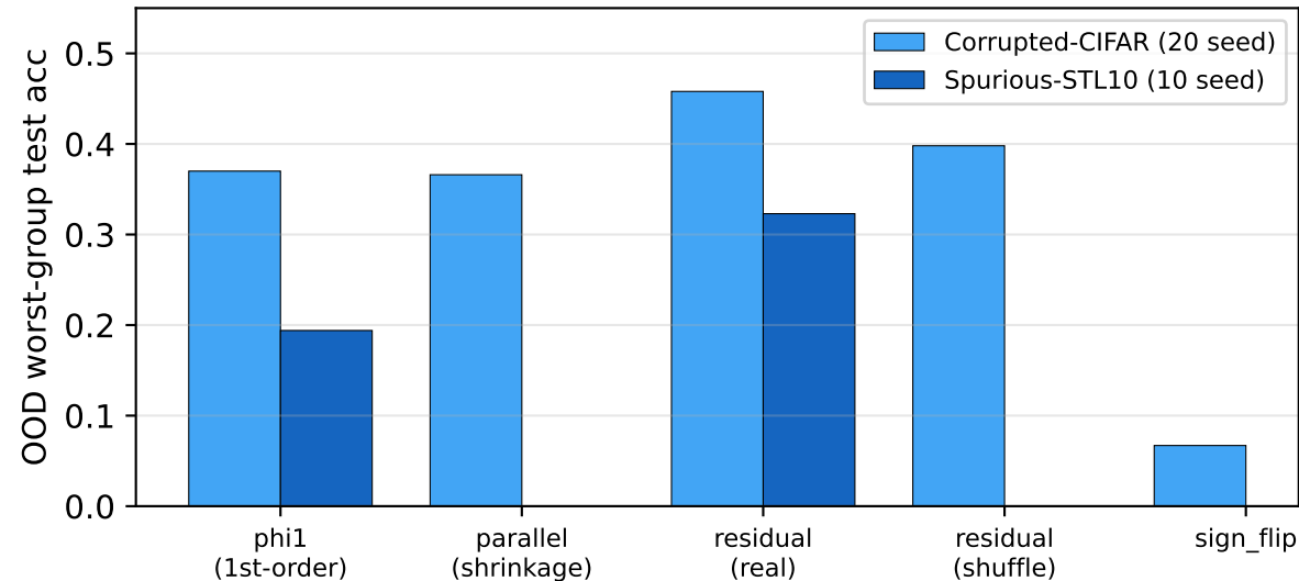
Cross-term decomposition: the orthogonal residual carries the 2nd-order signal real > shuffle > parallel; sign-flip collapses
