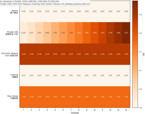
内存占用统计 / Memory Heatmaps: 3d-WindTurbineHub / physics_tet4
