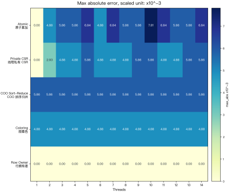
正确性统计 / Correctness Heatmaps: 3d-WindTurbineHub / physics_tet4
