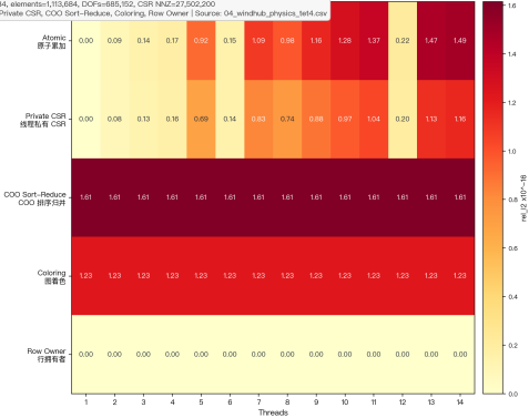
正确性统计 / Correctness Heatmaps: 3d-WindTurbineHub / physics_tet4
