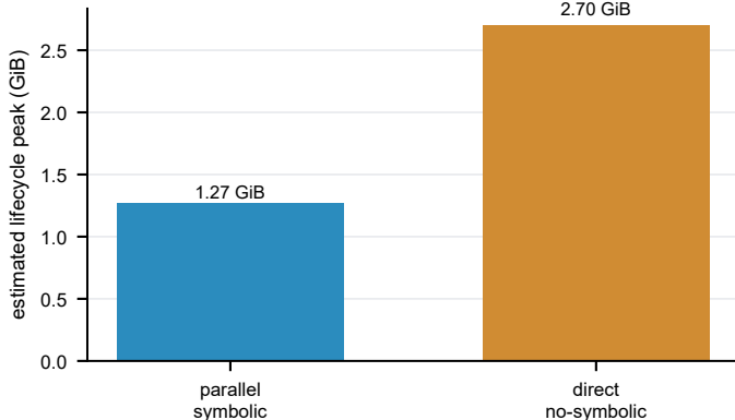
Modelled lifecycle peak at 8 threads
