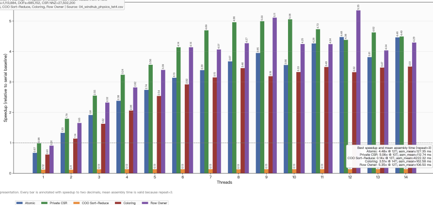
效率统计 / Efficiency Grouped Bars: 3d-WindTurbineHub / physics_tet4
