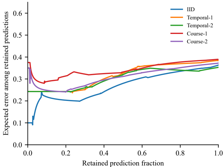
Logistic
