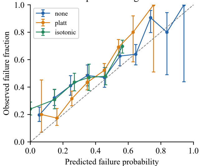
Temporal-2 / Logistic
