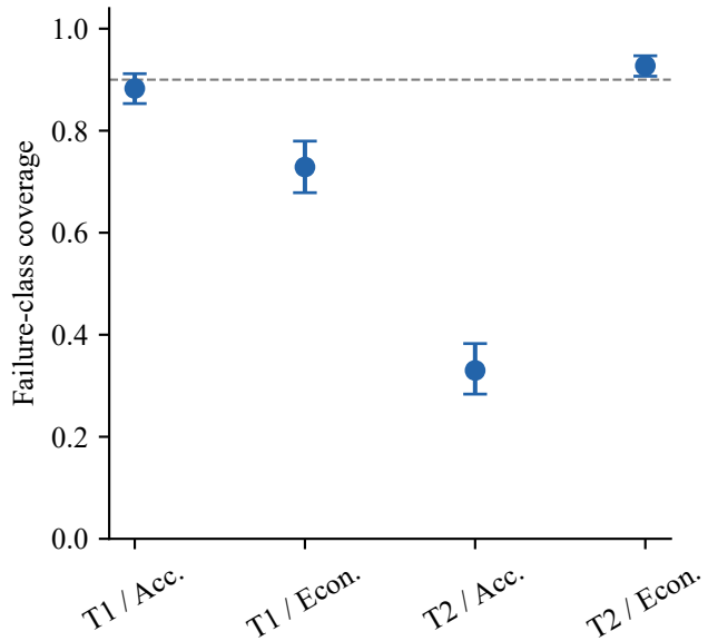
Logistic
