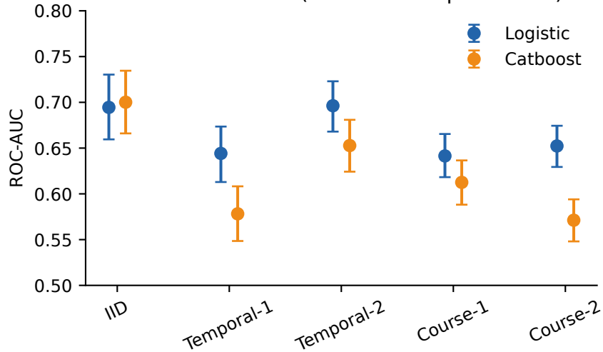
a Discrimination (95% bootstrap intervals)
