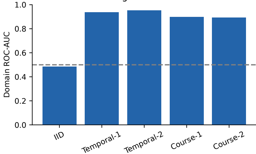
b Source-target feature differences
